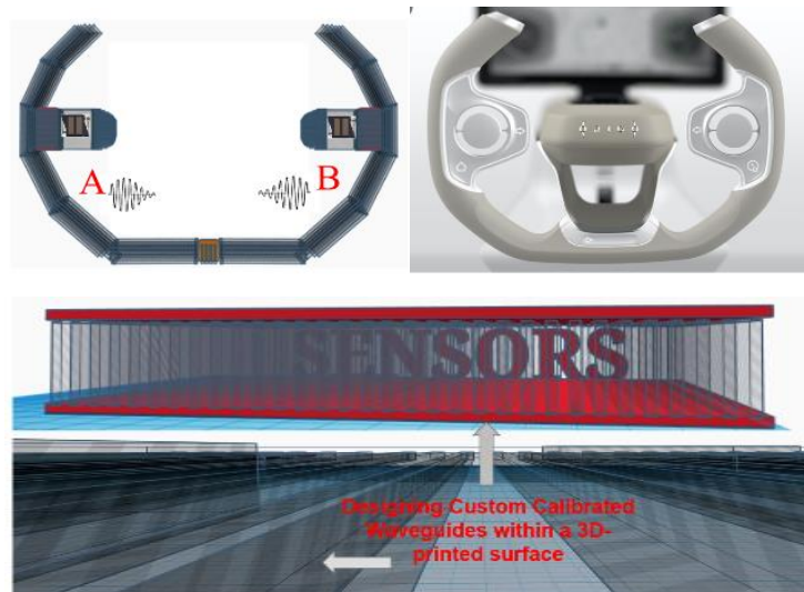
Figure 1. Design and structure of the Origo Embedded Haptic Waveguides and Constructive Wave Interference virtual exciter locations (A&B).
