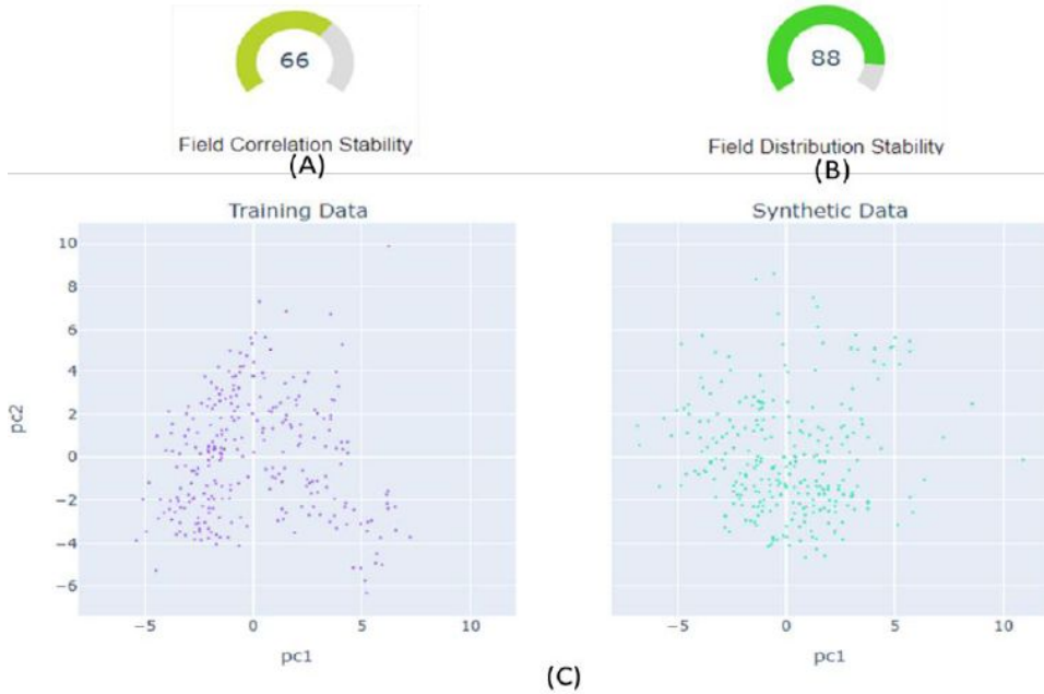
Figure 2: (A) Field correlation stability (B) field distribution stability (C) principal component analysis (PCA) of the real (training) and synthetic data of the tabular LSTM-GAN model respectively.
