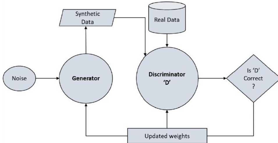
Figure 1: Framework of the GAN model used for synthetic data generation. Inspired by Li et al., 2021.
